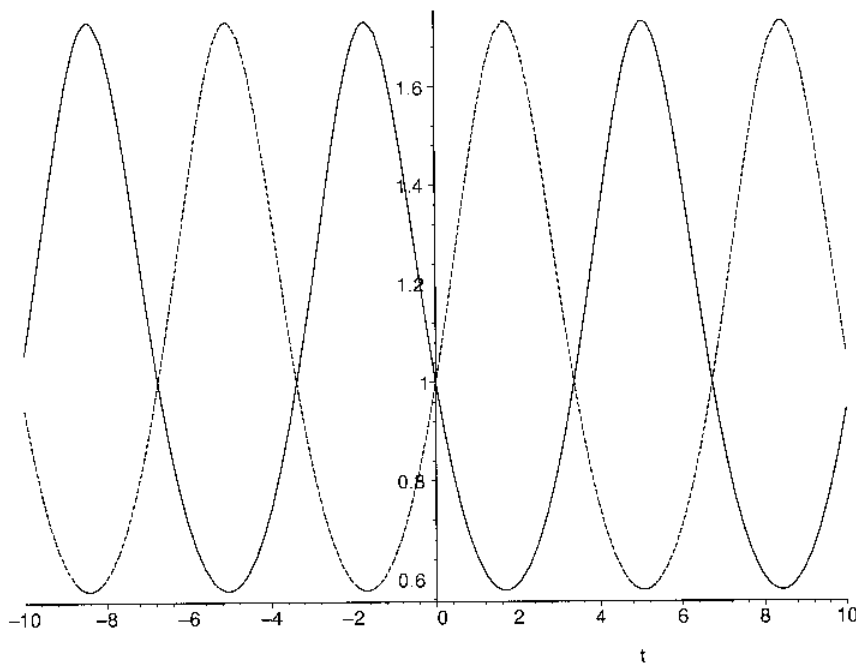
Fig. 3. Graphical presentations for solutions y_1 = \frac{dn(t, m)}{1 - msn(t, m)} (solid line) and y_2 = \frac{1 - msn(t, m)}{dn(t, m)} (dashed line) for m = 0.5 .
