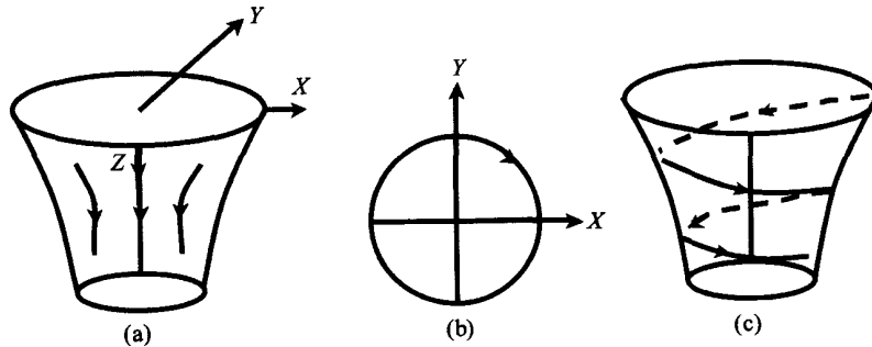
图1 龙卷风的速度场 (a)急流场; (b)涡旋场; (c)龙卷风场. Fig.1 Velocity of tornado
