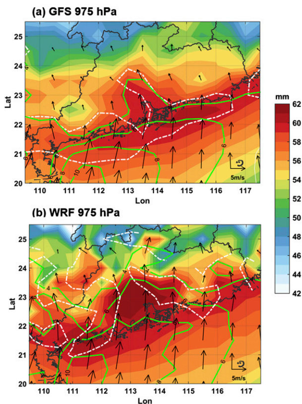
FIG. 17. Composite horizontal wind speed (contoured in green every 2 \text{ m s}^{-1} ), horizontal divergence of -1 \times 10^{-5} \text{ s}^{-1} (contoured in dashed white), horizontal wind vector at 975 hPa, and precipitable water (shaded every 1 mm) at the start time of LLJ-type episodes in (a) GFS analysis and (b) WRF simulations.
