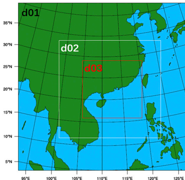
FIG. 3. WRF nested domains for the verification experiments.
