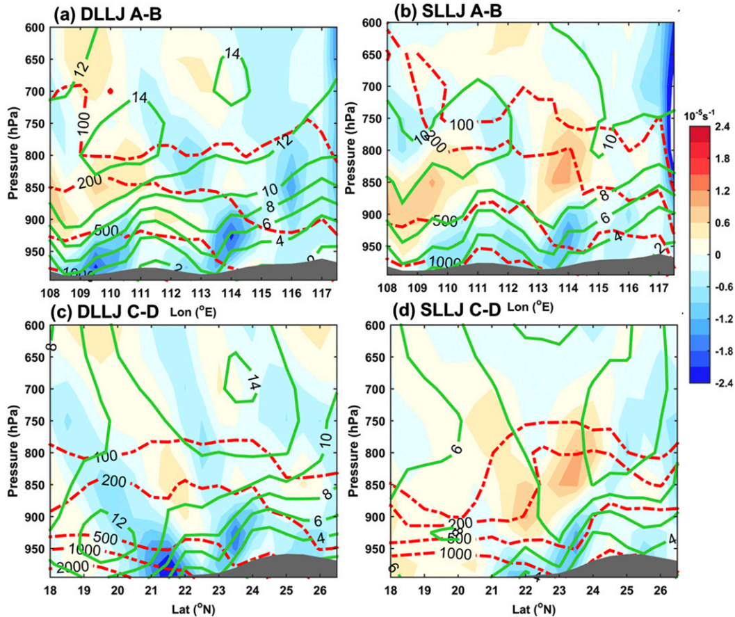
FIG. 11. Composite vertical cross sections at the start time of (a) DLLJ-type (path A–B in Fig. 9a) and (b) SLLJ-type (path A–B in Fig. 9b) warm-sector heavy rainfall episodes revealed by GFS analysis, including horizontal divergence (shaded every 0.3 \times 10^{-5} \text{ s}^{-1} ), horizontal wind speed (contoured every 2 \text{ m s}^{-1} in bold green), and CAPE (contoured at 100, 200, 500, 1000, and 2000 \text{J kg}^{-1} in dashed red). (c),(d) As in (a),(b), but for the vertical cross sections along path C–D given in Figs. 9c and 9d.
