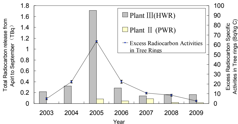
Figure 4 Comparison of excess ^{14}\text{C} in tree rings with ^{14}\text{C} discharges from Qinshan NPP (unpublished data provided by the nuclear power plant's operator). The ^{14}\text{C} discharge data of Plant II before 2004 and Plant I is absent.
