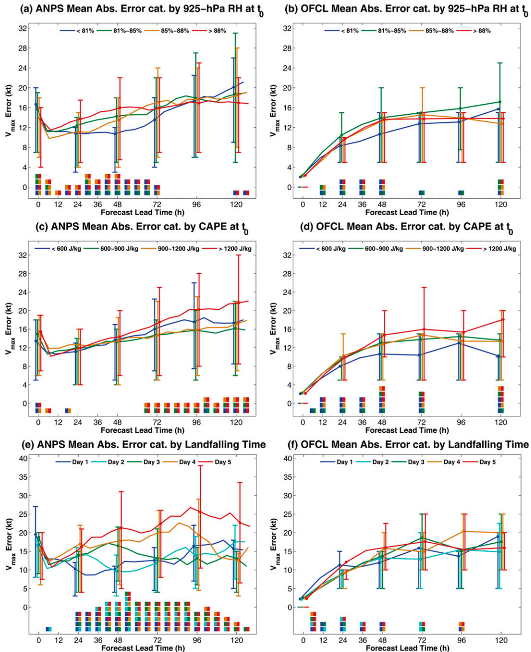
FIG. 10. As in Fig. 4, but for (a),(b) 925-hPa RH at forecast initialization time; (c),(d) CAPE and forecast initialization time; and (e),(f) days that the TC made landfall in best track during the forecast, for (left) ANPS and (right) OFCL forecasts.
