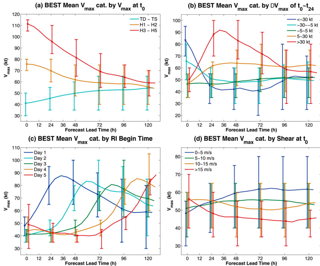
FIG. 6. Best-track mean intensity categorized by (a) best-track TC intensity categories at forecast initialization time, (b) best-track intensity changes during the first 24 h of forecasts, (c) days that rapid intensification began, and (d) 850–200-hPa vertical wind shear magnitudes. The vertical lines accompanying intensity trends are ranges between the first and the third quartiles of each group every 24 h.
