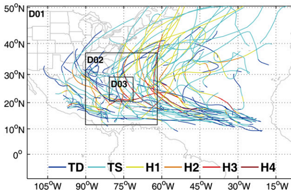
FIG. 1. Domain setting as of 0000 UTC 26 Oct 2012 used for a forecast of Hurricane Sandy (2012) with tracks of all simulated TCs during 2008–12. Different colors of tracks stand for different hurricane intensity categories as labeled at the bottom of this figure.
