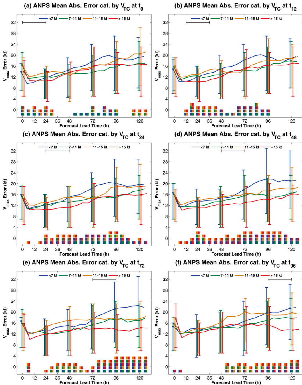
FIG. 11. As in Fig. 4, but for the best-track translation speed of the TC at forecast lead times of (a) 0, (b) 12, (c) 24, (d) 48, (e) 72, and (f) 96 h for ANPS forecasts. The horizontal range lines at the top indicate 0–24-h time period after categorization time.
