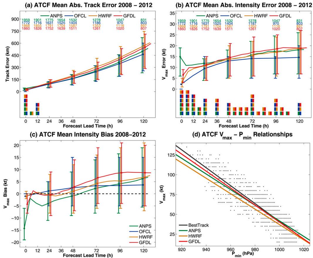
FIG. 2. Mean absolute errors during 2008–12 of (a) track and (b) maximum wind speed ( V_{max} ) for selected regional NWP models and NHC official forecasts, as well as (c) mean biases of V_{max} and (d) relationships between V_{max} and P_{min} for NWP model forecasts and best-track observations. In (a) and (b), the numbers at the top indicate the sample size of different models at that time, the two-color squares at the bottom indicate significantly different pairs at that time. In (a)–(c), the vertical lines accompanying error or bias trends are ranges between the first and the third quartiles of each group every 24 h. In (d), the scatters are each single V_{max} – P_{min} pair of best track.
