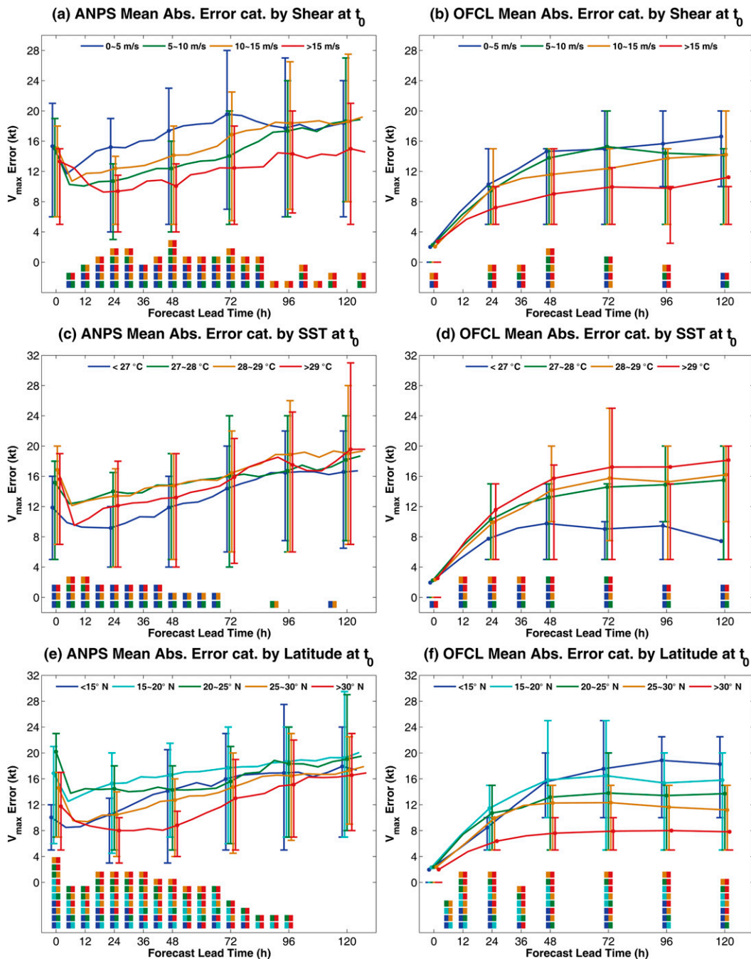
FIG. 8. As in Fig. 4, but for (a),(b) 850–200-hPa vertical wind shear magnitudes; (c),(d) SST at forecast initialization time; and (e),(f) center latitude at forecast initialization time, for (left) ANPS and (right) OFCL forecasts.
