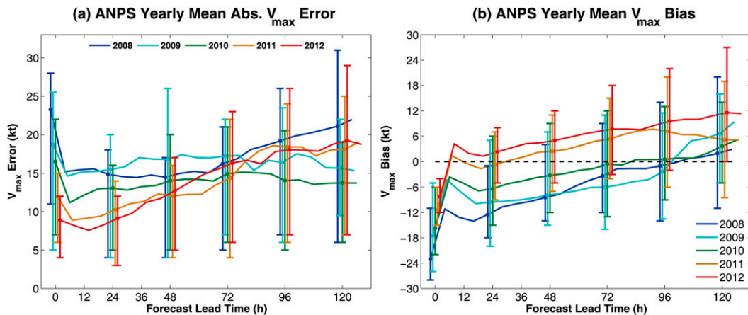
FIG. 3. (a) Yearly mean absolute intensity forecast errors and (b) yearly mean intensity biases of ANPS. The vertical lines accompanying error or bias trends are ranges between the first and the third quartiles of each group every 24 h.
