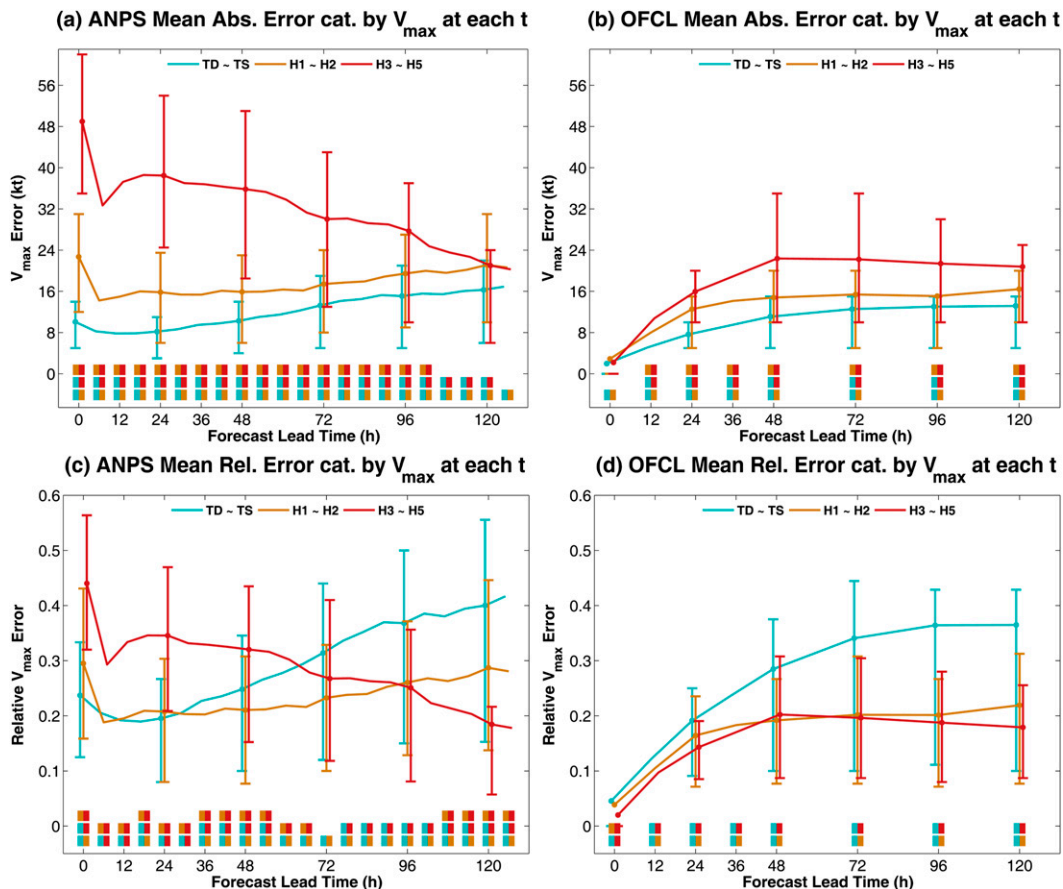
FIG. 5. As in Fig. 4, but for (a) ANPS and (b) OFCL mean absolute intensity forecast errors, and (c) ANPS and (d) OFCL mean relative intensity forecast errors, all categorized by best-track TC intensity categories at each verification forecast lead times.
