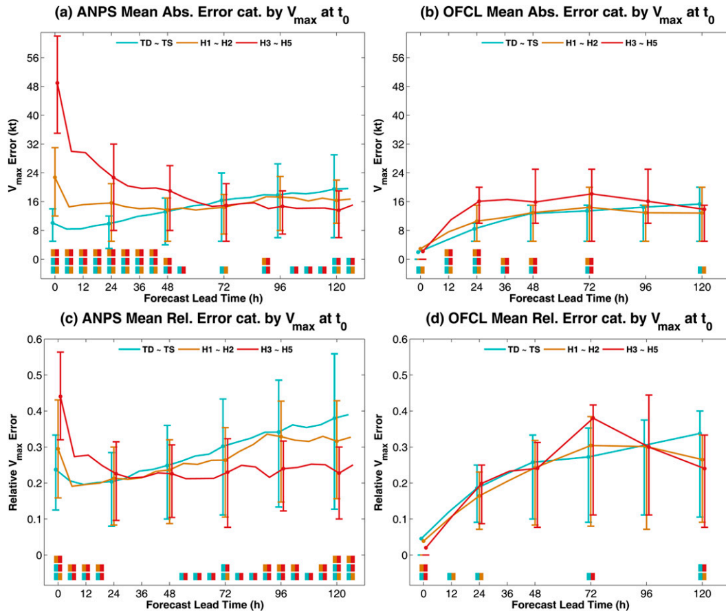
FIG. 4. (a) ANPS and (b) OFCL mean absolute intensity forecast errors, and (c) ANPS and (d) OFCL mean relative intensity forecast errors, all categorized by best-track TC intensity categories at forecast initialization time ( t = 0 h). The vertical lines accompanying error trends are ranges between the first and the third quartiles of each group every 24 h; the two-color squares at the bottom indicate significantly different pairs at that time.
