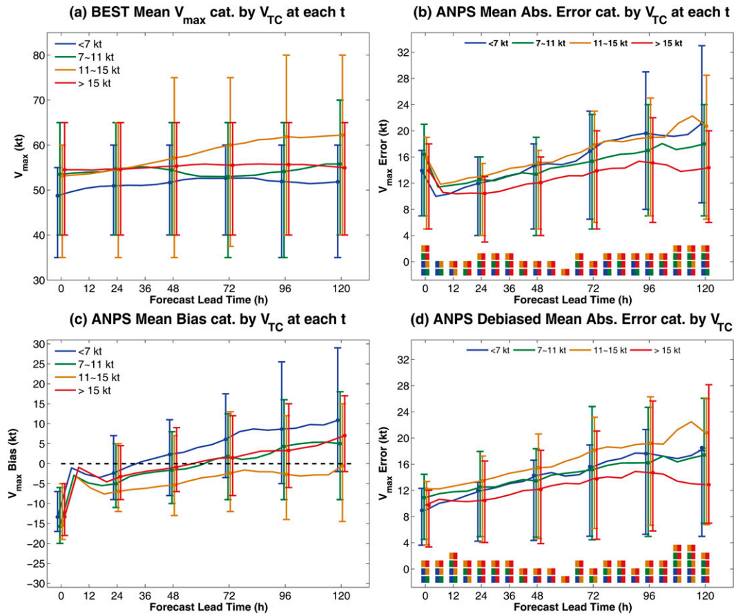
FIG. 12. (a) Best-track mean intensity, (b) ANPS mean absolute intensity forecast errors, (c) ANPS mean intensity forecast bias, and (d) ANPS debiased mean absolute intensity forecast errors, all categorized by translation speed of the TC at each verification forecast lead times. The vertical lines accompanying intensity, error or bias trends are ranges between the first and the third quartiles of each group every 24 h. In (b) and (d), the two-color squares at the bottom indicate significantly different pairs at that time.
