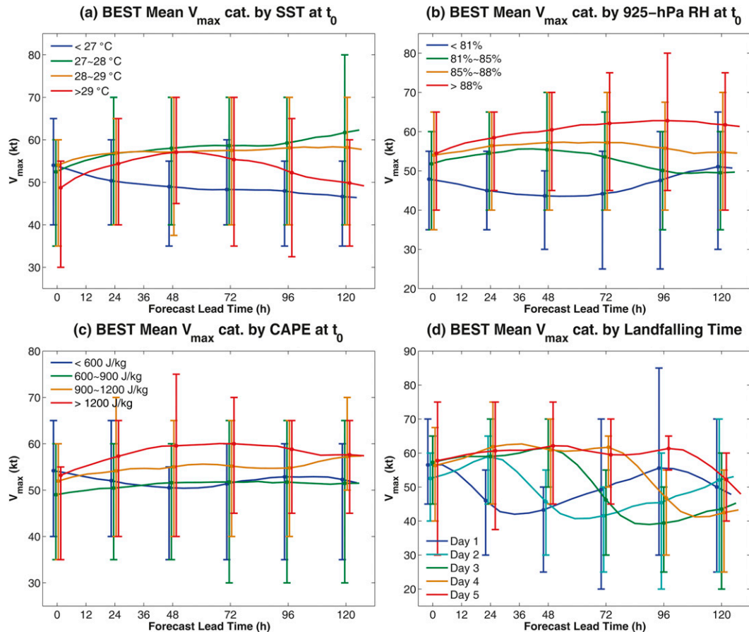
FIG. 9. As in Fig. 6, but for (a) SST at forecast initialization time, (b) 925-hPa RH at forecast initialization time, (c) CAPE at forecast initialization time, and (d) days that the TC made landfall in best track during the forecast.
