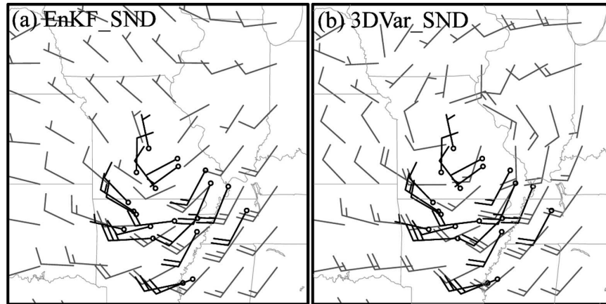
FIG. 7. Wind vector forecast (gray color) at 700 hPa of (a) EnKF_SND and (b) 3DVAR_SND valid at 1730 UTC 11 Jun 2003 starting from their respective posteriors at 1112 UTC 11 Jun. The drosonde observation during 1604–1905 UTC 11 Jun are plotted in black.
