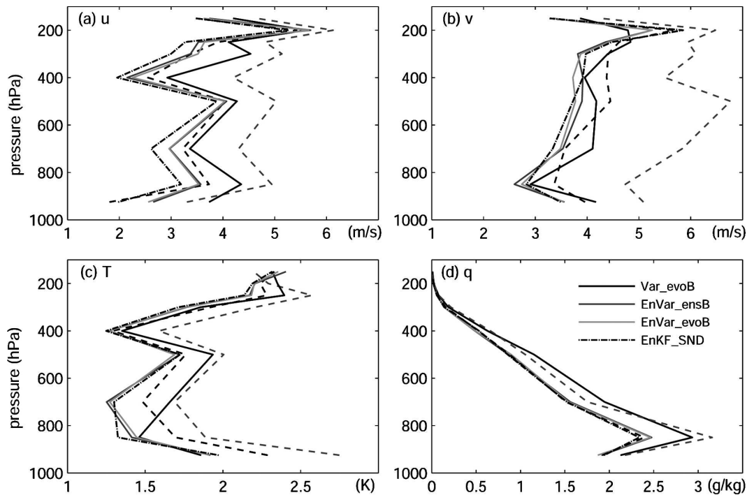
FIG. 16. Vertical distributions of the horizontally averaged prior RMSEs of (a) u , (b) v , (c) T , and (d) q at 36 h in Var_ovoB (black solid), EnVar_ensB (gray solid), and EnVar_ovoB (light gray solid) in comparison with EnKF_SND (black dot-dashed). Also plotted are the RMSEs of the reference forecast DF (gray dashed) and EF (black dashed).
