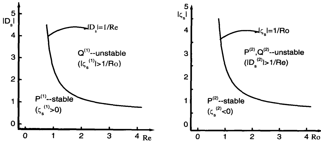
Fig. 2. The bifurcation curves under the action of \zeta D .
