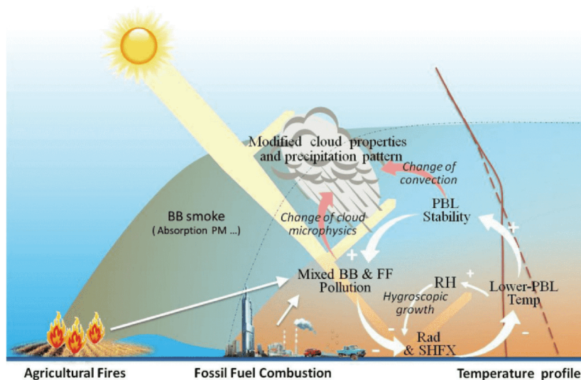
Figure 17 A schematic of interactions of air pollution-PBL dynamics and aerosol-radiation-cloud interaction under a condition of mixed agriculture burning plumes and fossil fuel combustion pollutants. Note: yellow bands show the radiative transfer of solar radiation. The brown solid and dashed lines denote the air temperature profiles for episode and non-episode cases, respectively. The black thin dashed line represents the top of fossil fuel combustion plume under a non-episode condition. The plus (+) and minus (-) signs denote enhancement and reduction of a target process, respectively. Adapted from Ding et al. (2013).
