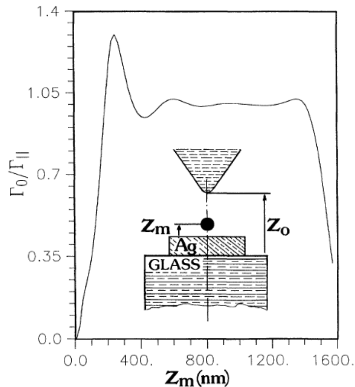
FIG. 2. Distance dependence of the normalized lifetime \Gamma_0/\Gamma_{||} inside the junction, as a function of the position of the molecule. The geometry used in the simulation is described in the inset and the tip-sample separation is maintained at Z_0 = 1600 nm. The glass sample is covered with a square shaped silver layer 300 nm long and 20 nm high.
